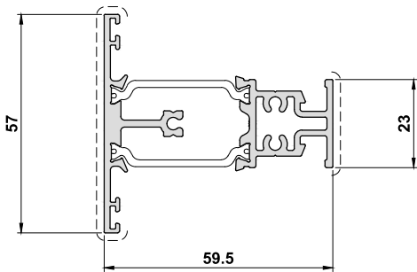
ETC4132 / G ETC4124 Dummy Transom
