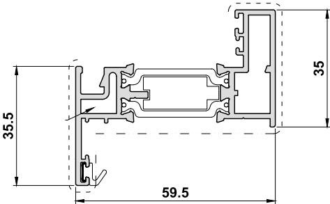
ETC4120 / G Externally Beaded Sash
