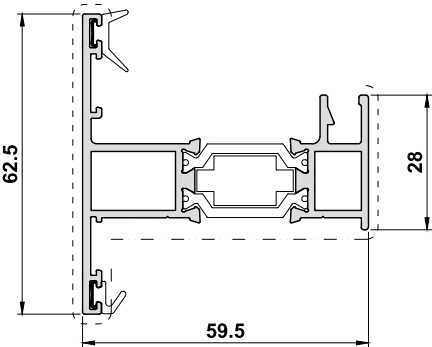
ETC4129 / G Internally Bead Sash
