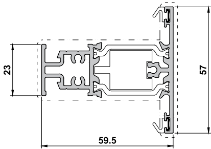
ETC4130 / G Transom/Mullion
