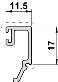
ETC4179 11.5mm Bead
