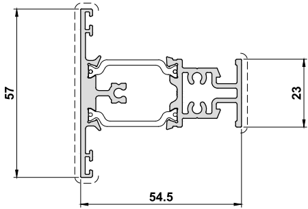
ETC4133 / G ETC4125 Dummy Transom
