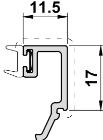
ETC4179G 11.5mm Bead with Gasket
