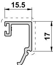
UN3164 15.5mm Bead
