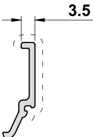
UN3168 3.5mm Bead
