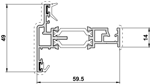
ETC4125 / G Heritage Sash for 24mm Glazing Only
