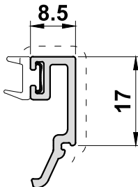
UN3166G 8.5mm Bead with Gasket
