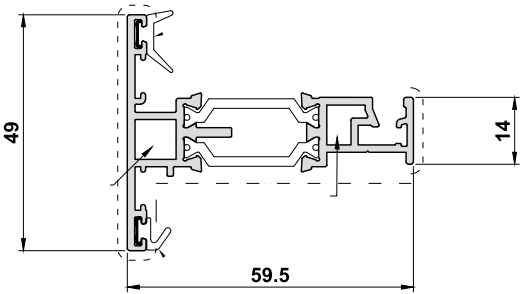
ETC4124 / G Slimline Sash
