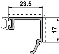
UN3162G 23.5mm Bead with Gasket
