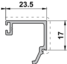
UN3162N 23.5mm Bead
