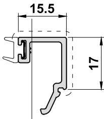
UN3164G 15.5mm Bead with Gasket
