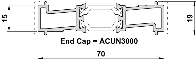
UN3000 Flush Horizontal Coupler
