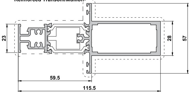
ETC4136 Reinforced Transom/Mullion
