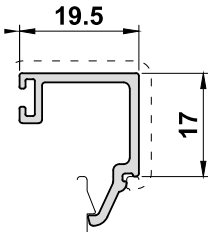
UN3160 19.5mm Bead
