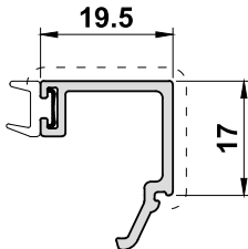
UN3160G 19.5mm Bead with Gasket
